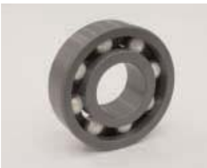
Full Ceramic Bearing Silicon nitride inner and outer ring. Silicon nitride rolling element. Zirconia ball.
